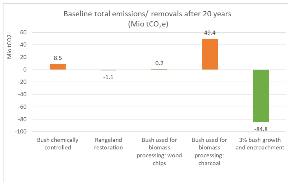
Figure 13: Overview total emissions and removals of baseline bush control activities compared to carbon sink of bush growth and encroachment over 20 years; values are given in Mio tCO 2 e, negative values indicate carbon removals.
