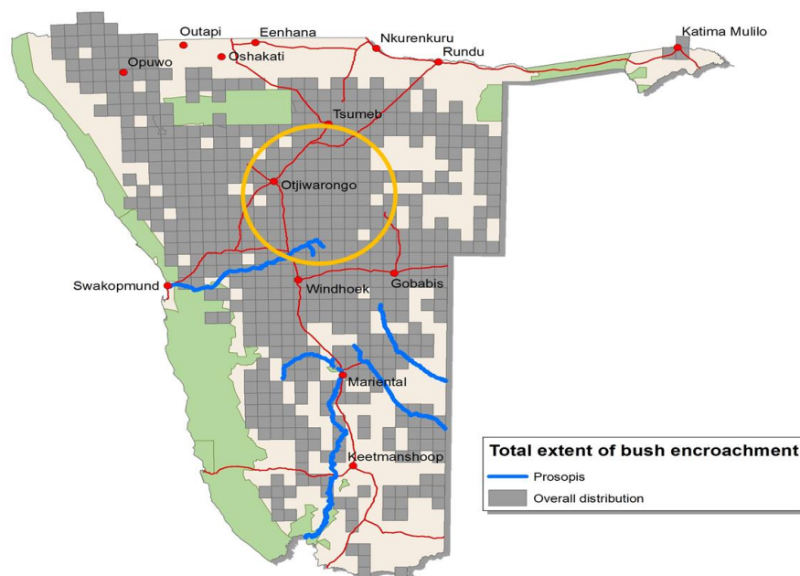
Figure 8: Study assessment area (yellow circle) and extent of bush encroached areas in Namibia
